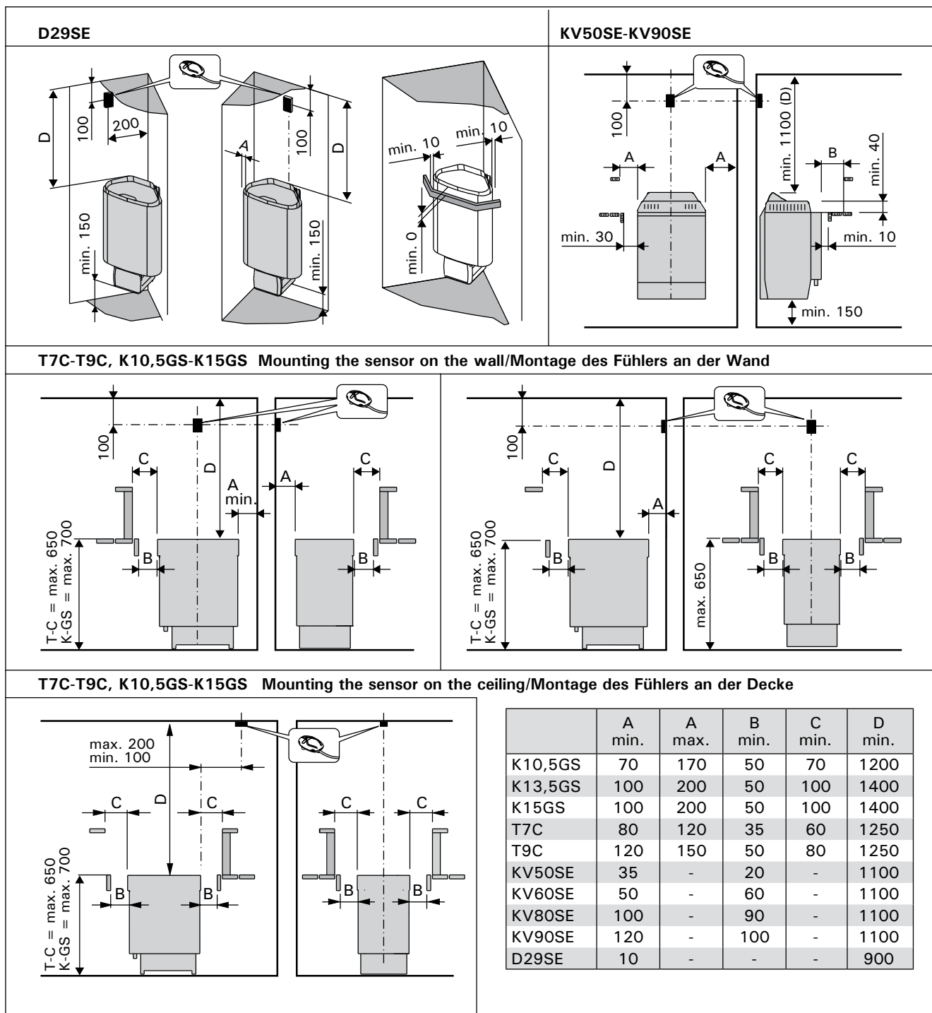
Figure 5. Safety distances (all dimensions in millimeters)
