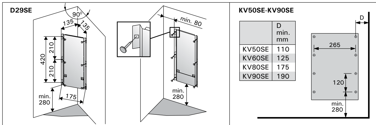
Figure 6. Location of the mounting rack of the heater (all dimensions in millimeters)
