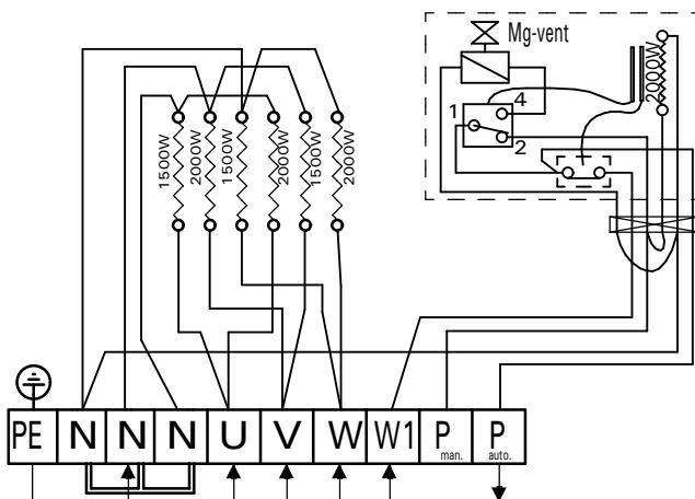
Figure 9. Electrical connections Abbildung 9. Elektroanschlüsse
