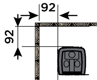
SAFETY DISTANCES TO THE WALLS
