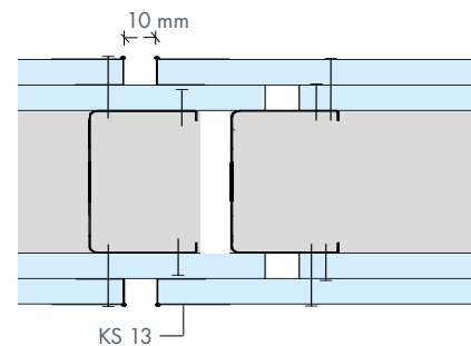
Princip for lodret dilatationsfuge. Brand: EI 60 A2-s1, d0
